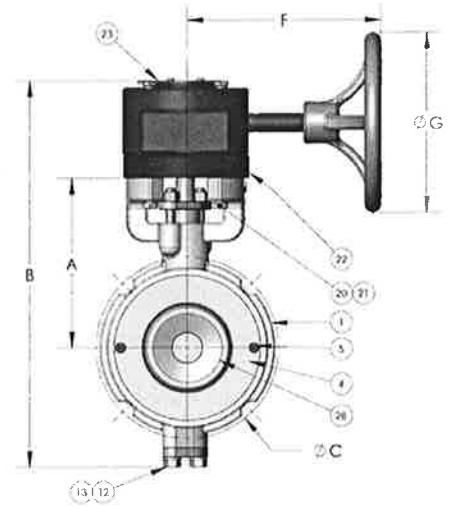
3" 150/300 HP WAFER SHOWN
