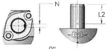
8" STEM DETAIL
