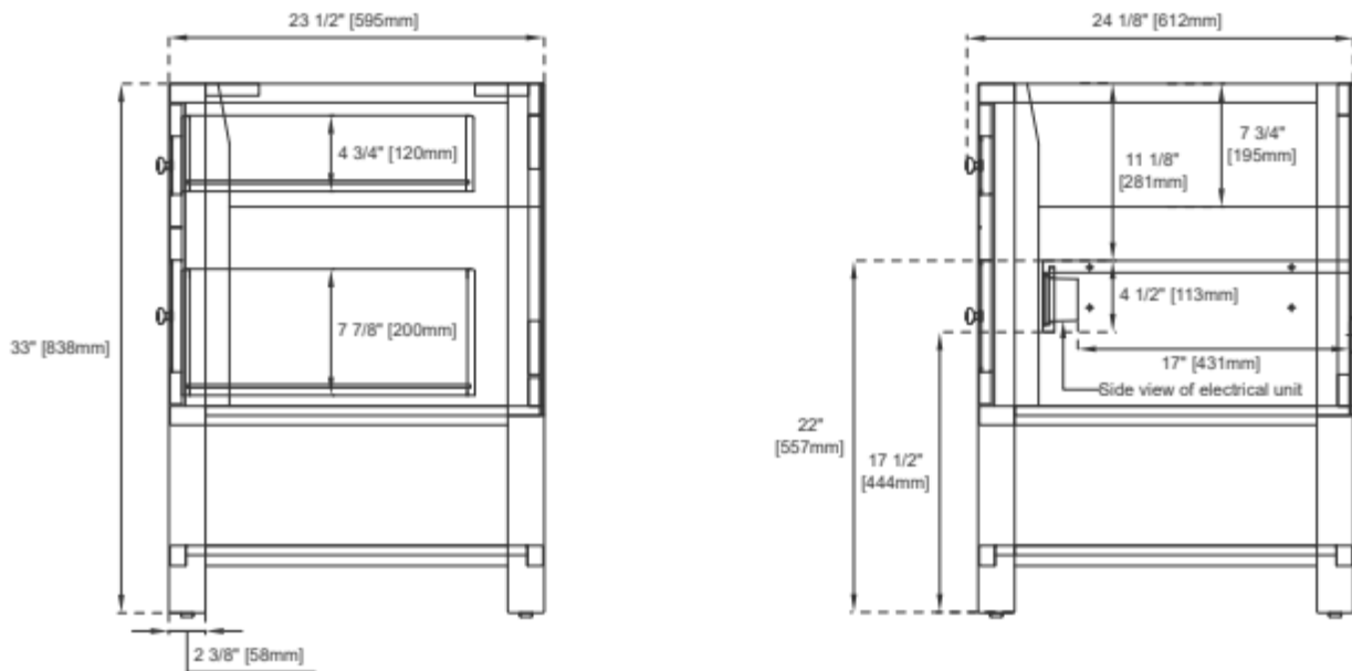
Side View
