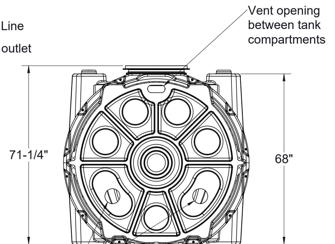
SECTION B-B
