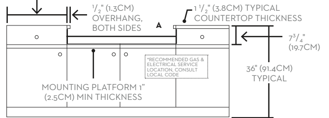
CABINET / COUNTERTOP DIMENSIONS - FRONT VIEW
