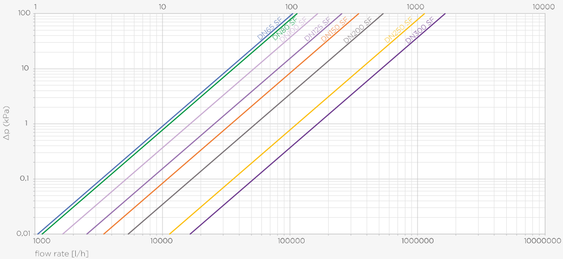
pressure loss Apollo ProFlow V955
