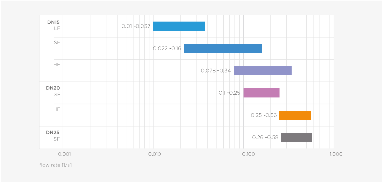
flow rate Apollo ProFlow PSUI600 PICV
