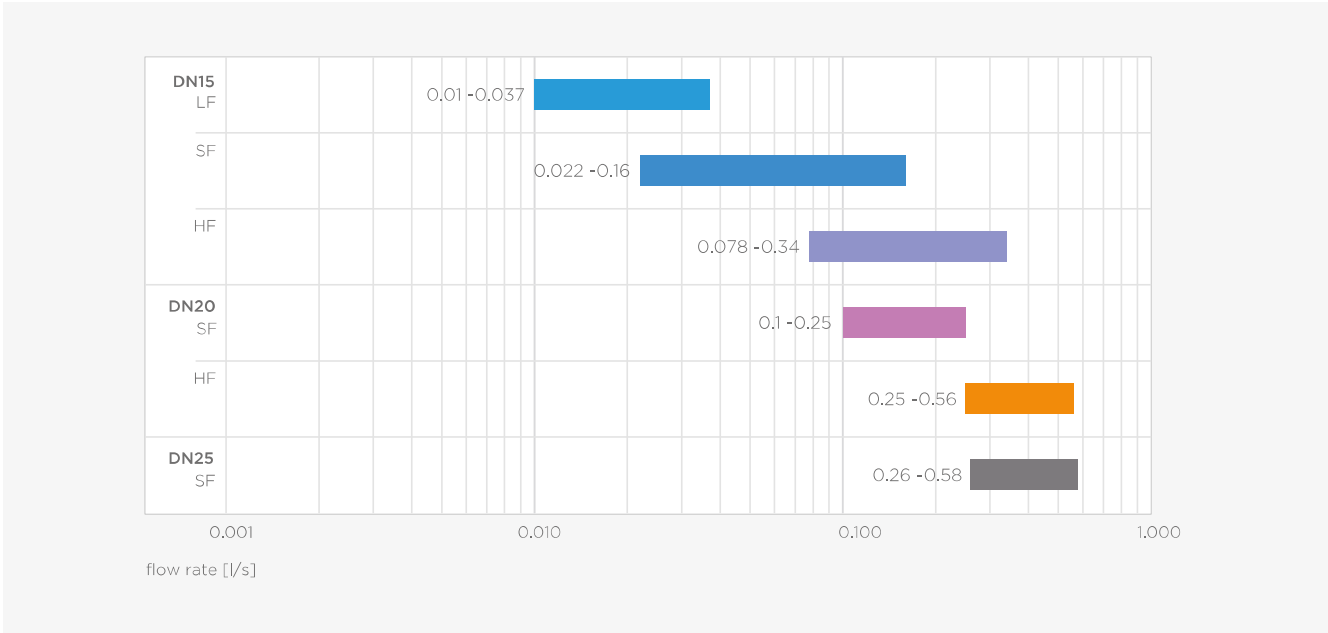
flow rate Apollo ProFlow PS1600 PICV
