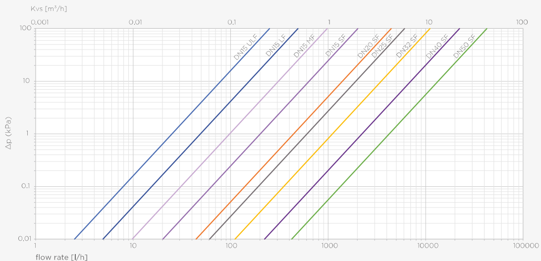
pressure loss Apollo ProFlow 1260
