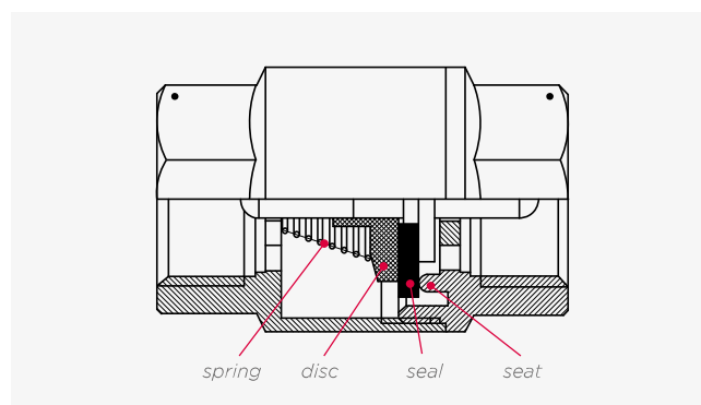
spring check valve principle
