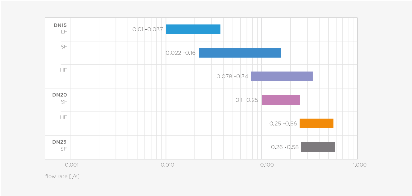
flow rate Apollo ProFlow 1600 PICV
