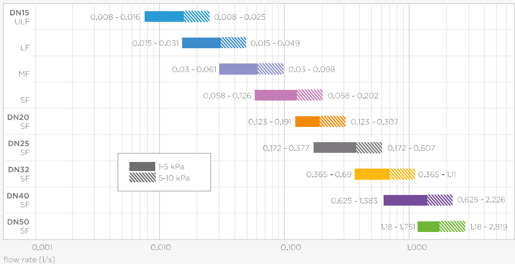
flow rate Apollo ProFlow PS1260
