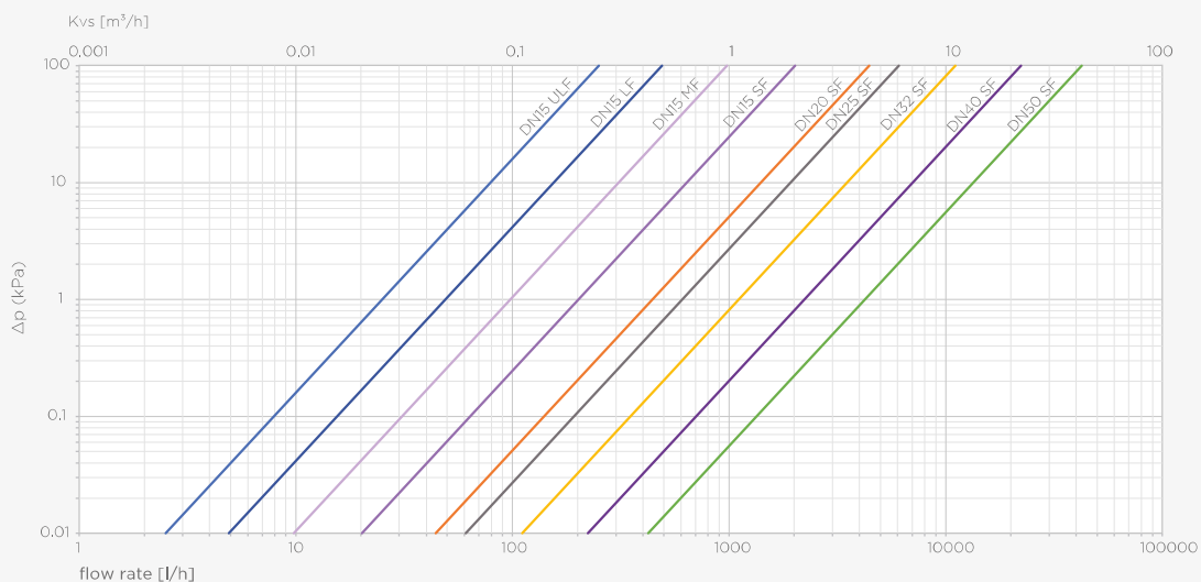
pressure loss Apollo ProFlow PSU1260
