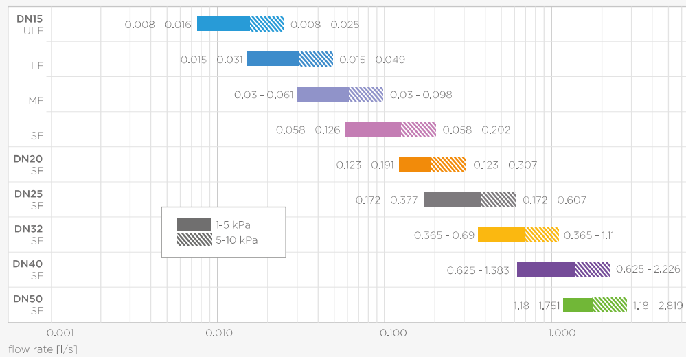
flow rate Apollo ProFlow PSU1260
