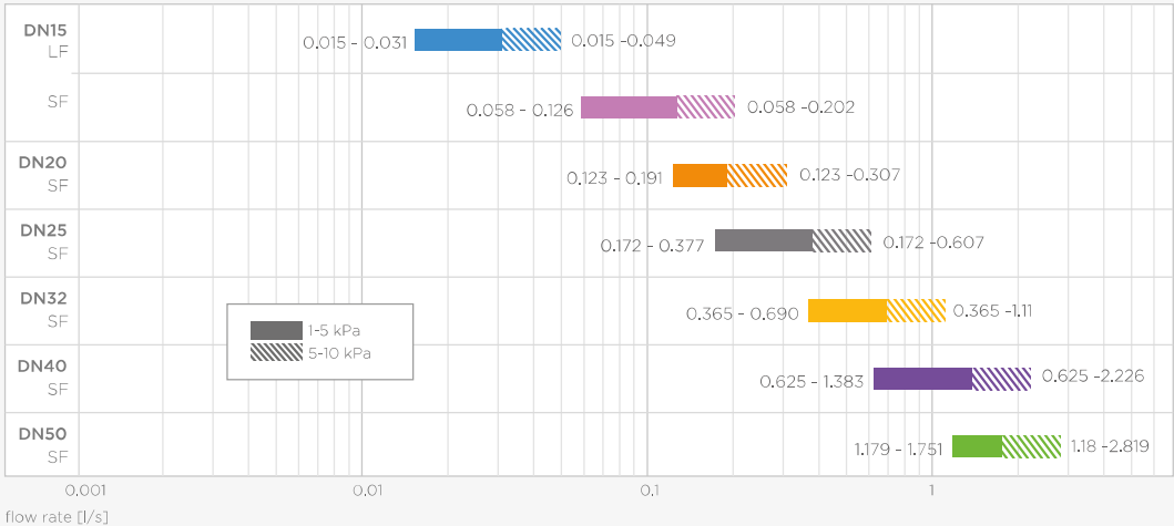
flow rate Apollo ProFlow PP1260
