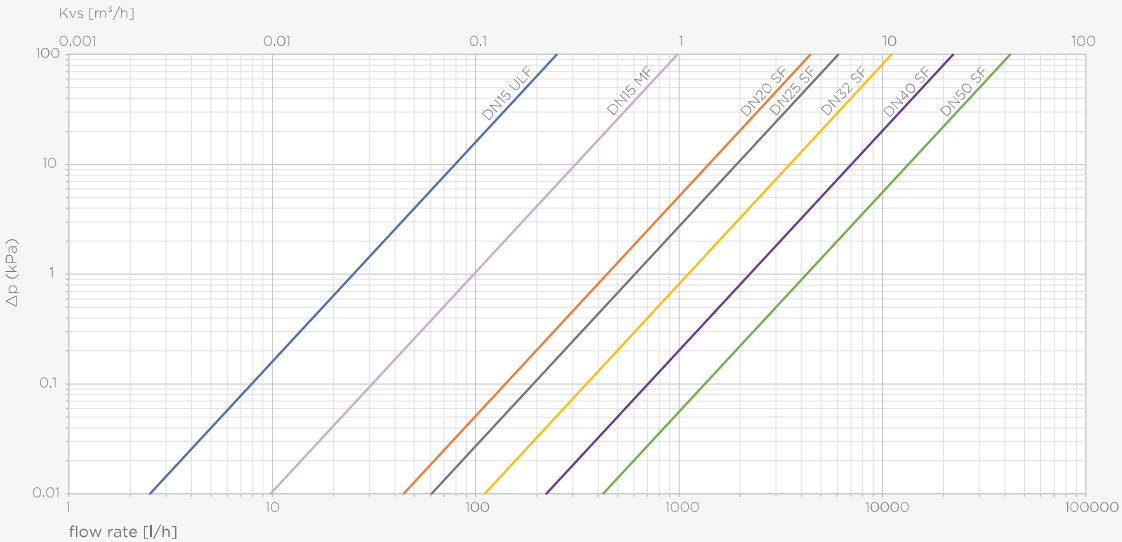
pressure loss Apollo ProFlow PP1260
