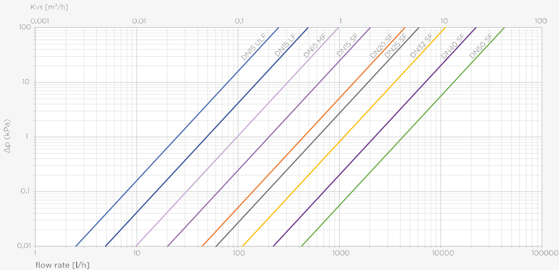
pressure loss Apollo ProFlow PS1260
