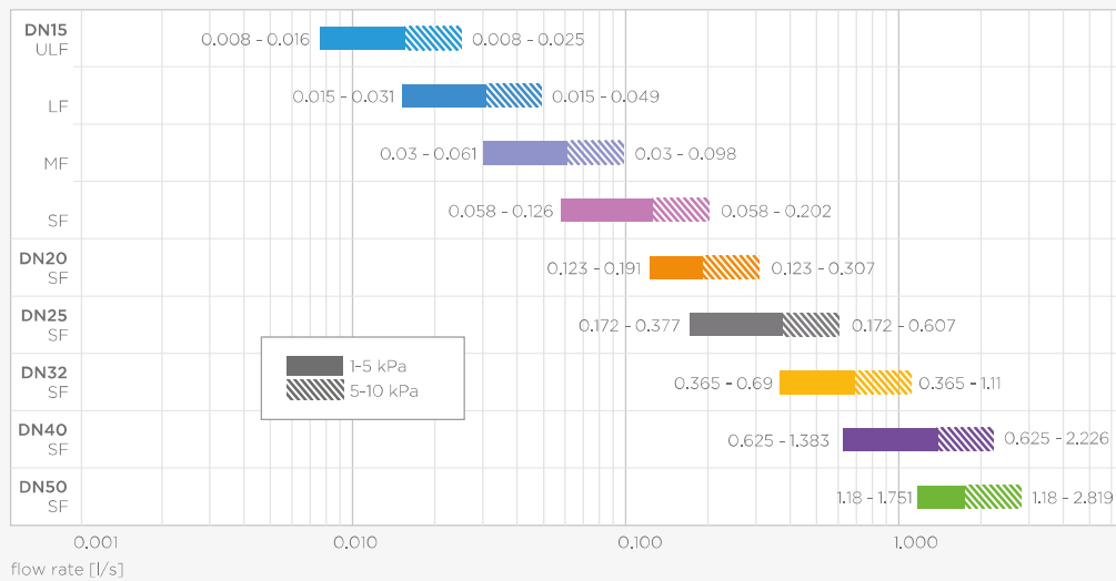
flow rate Apollo ProFlow 1260
