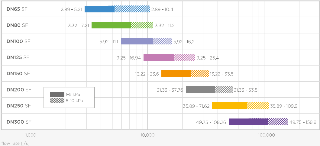
flow rate Apollo ProFlow V955
