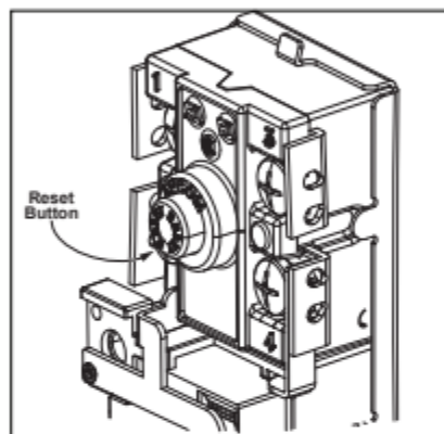
Figure 25 - Energy Cut Off (ECO) button
