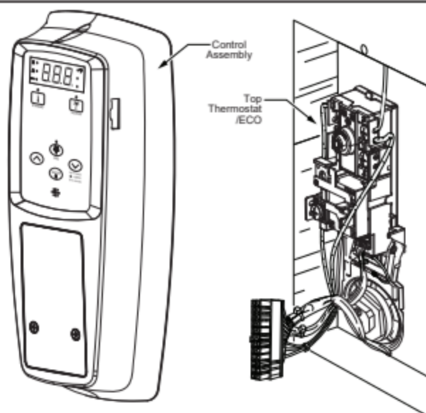
Figure 21 - Control Assembly
