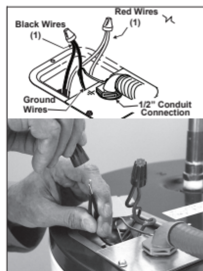
Figure 19 - Connecting the electrical wires.
