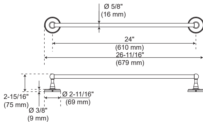
18" Towel Bar
