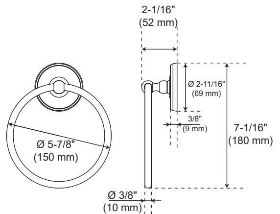
Towel Ring
