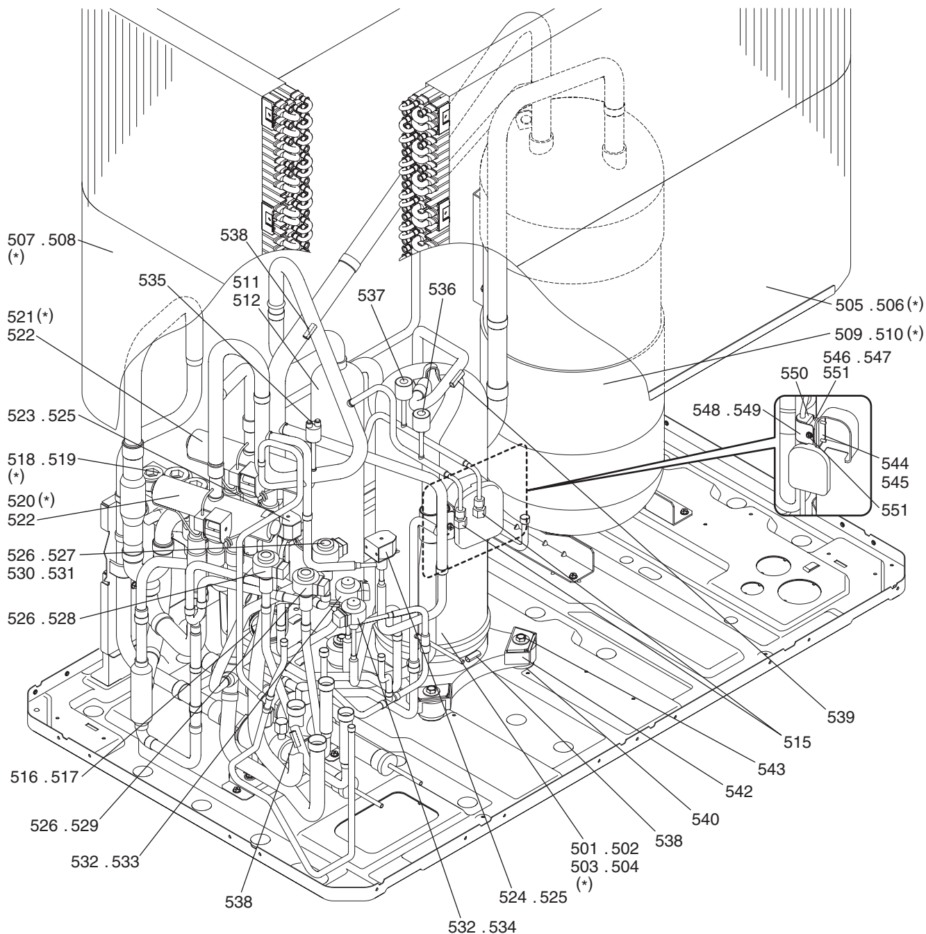
PURY-EP96,EP120TNU-A(-BS) PURY-EP96,EP120YNU-A(-BS)
