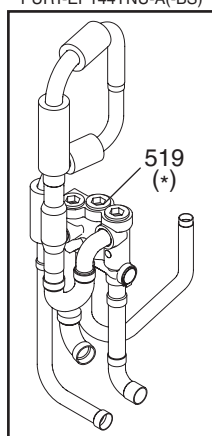
PURY-EP144TNU-A(-BS) PURY-EP144YNU-A(-BS)
