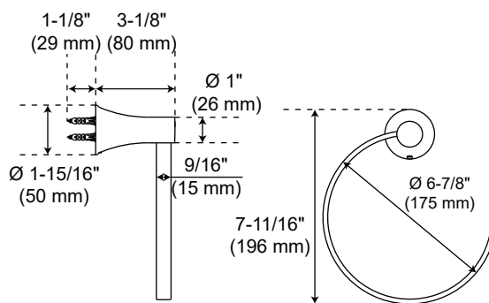
Towel Ring
