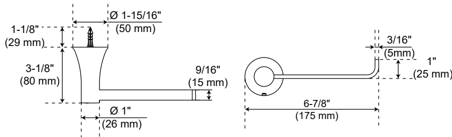
Tissue Holder
