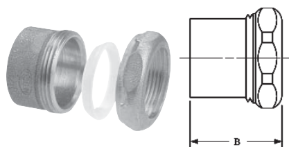
801-2-7 DWV Fitting Trap Adapter Ftg x SJ – Cast
