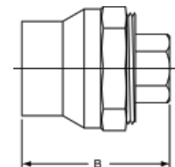
816 DWV Fitting Cleanout Ftg x Cleanout w/Plug – Cast
