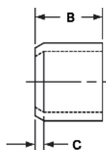
901-2-F DWV Fitting Flush Bushing Ftg x C – Wrot
