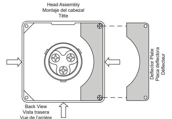
Figure 12 - Optional Deflector
