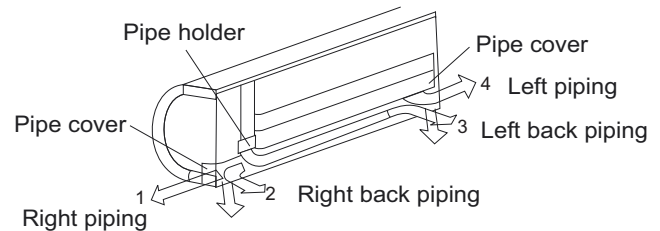
Fig. 4 — Piping Locations
