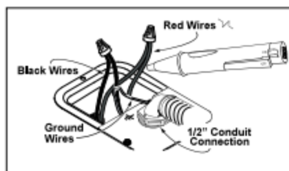
Figure 39 - Non-Contact Circuit Tester
