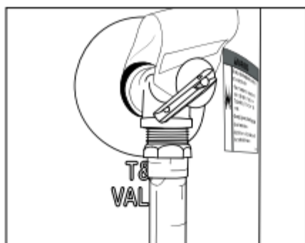
Figure 11 - The T&P Relief Valve discharge pipe must be installed properly and piped to an adequate drain.
