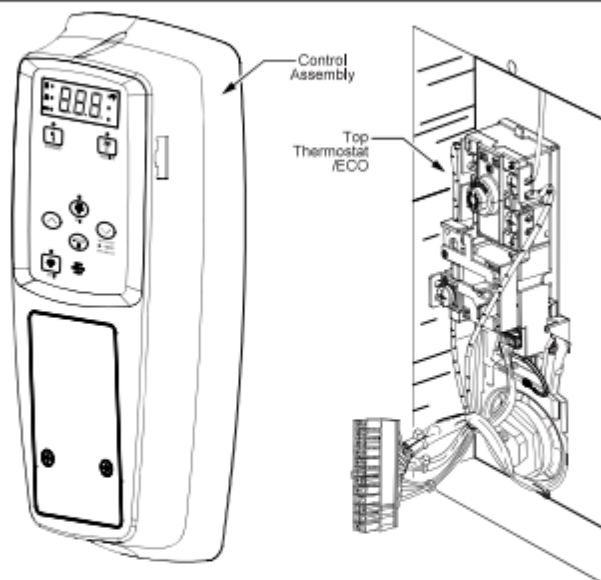
Figure 20 - Control Assembly
