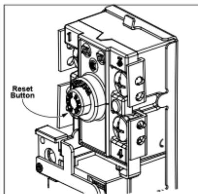
Figure 27 - Energy Cut Off (ECO) button
