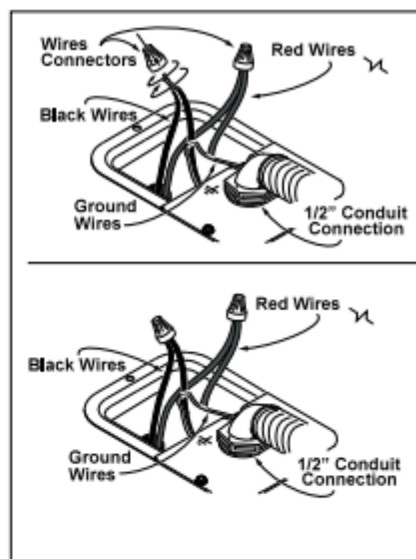
Figure 18 - Connecting the electrical wires.
