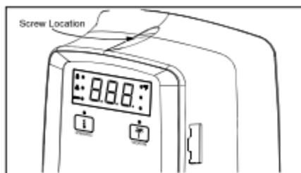
Figure 36 - Control Assembly
