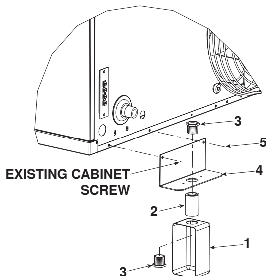
Figure 17. Thermostat Bracket Kit (Refer to Table 32 )
