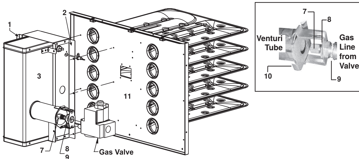
Figure 7. Replacement Heat Exchanger and Burner Assembly Components (Refer to Table 15 and Table 16 )
