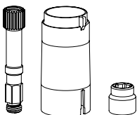
Spindle extension Spare part. Included in valve sizes 2 1/2" - 6". Needed on sizes 2 1/2" - 6" when using TA prefab insulations (52 189-8xx).
