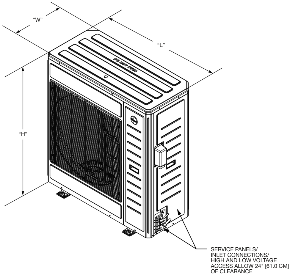
Illustration A1345-02-00
