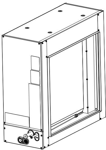
Fig. 1 – ESH5X Coil
