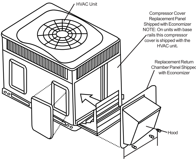
Vertical Economizer
