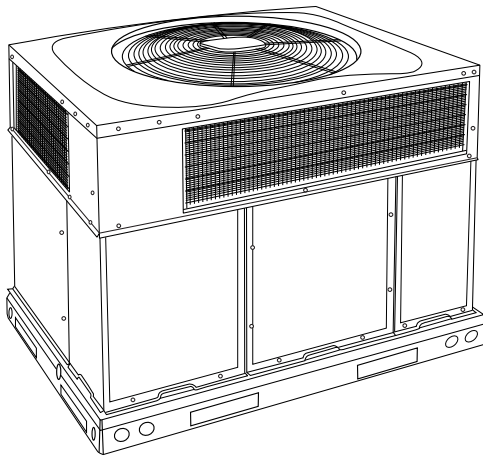
Fig. 1 – Unit PGB4 (Low NOx Model Available)
