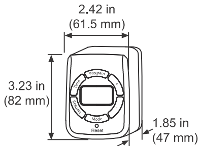
Fig. 6 Digital timer dimensions
