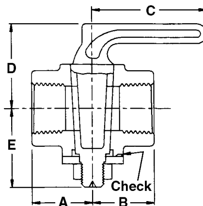
1/2" & 3/4" bottom check
