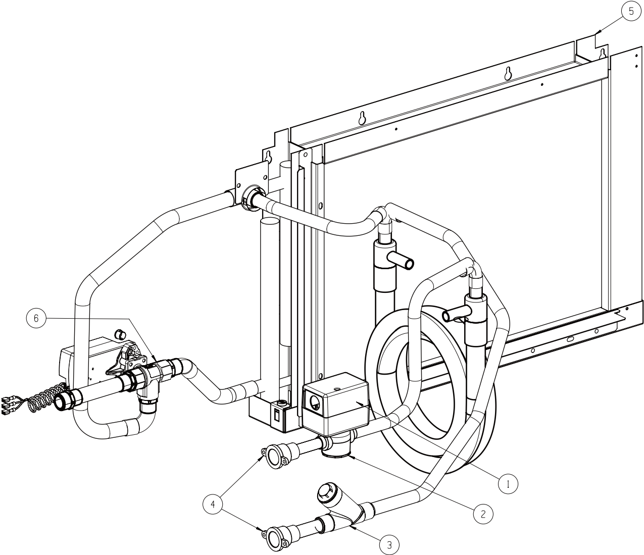
Waterside Economizer With 3 Way Valve and Controls
