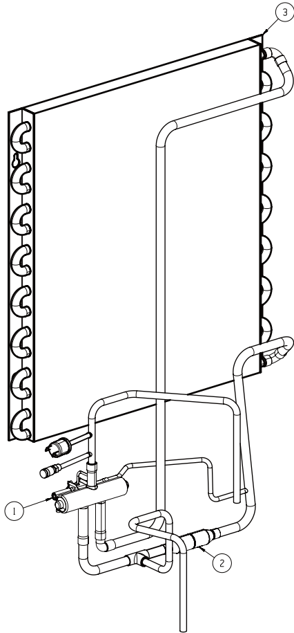
Hot Gas Reheat
