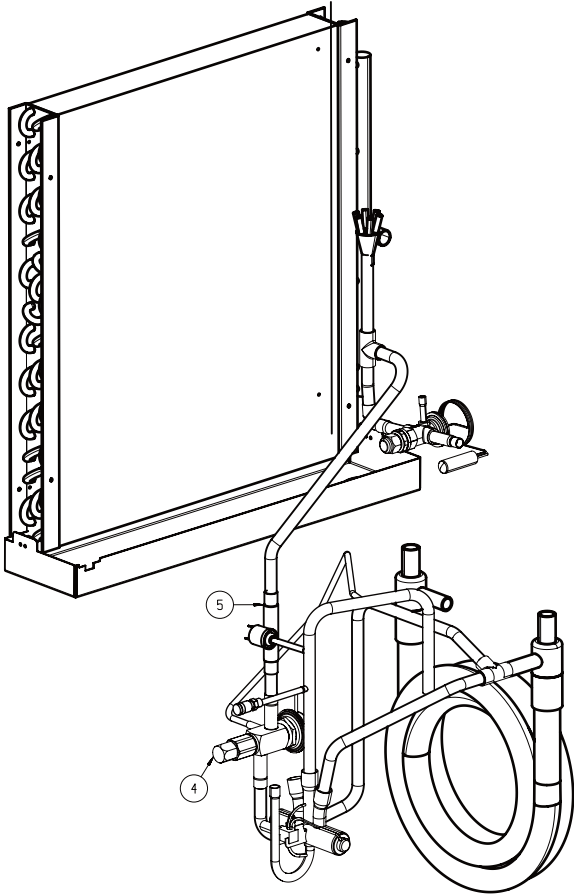
Hot Gas Bypass
