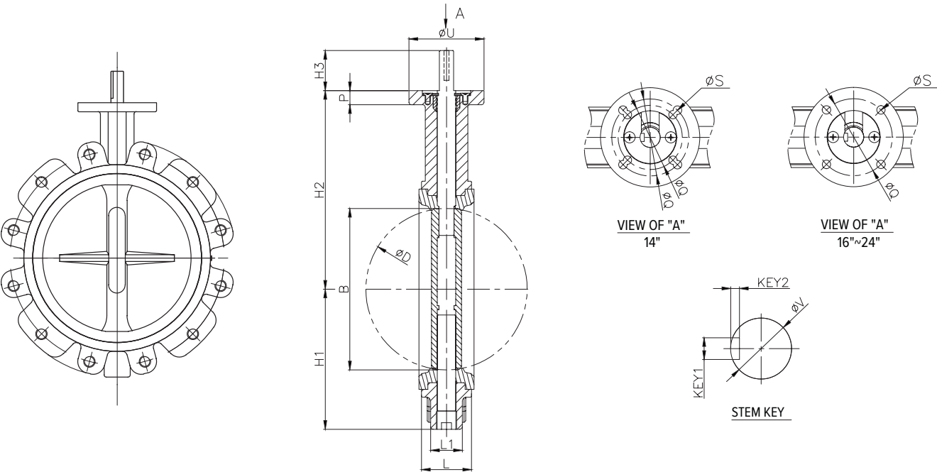
DIMENSIONS 14" – 24" (INCHES)
