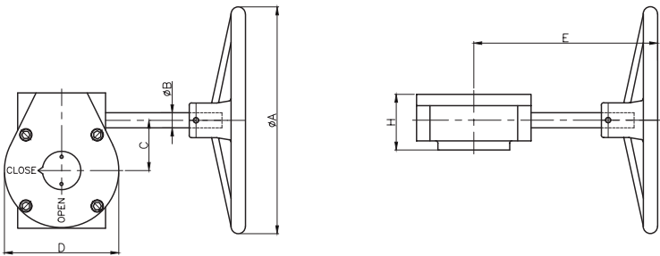
DIMENSIONS (MILIMETERS)
