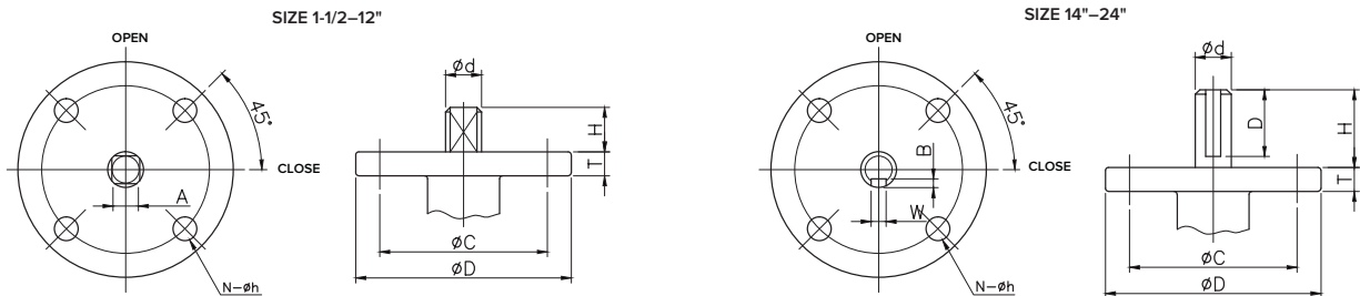
DIMENSIONS 2" – 24" (INCHES)
