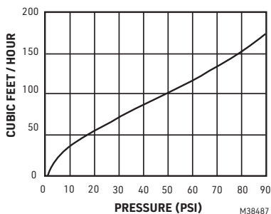
Fig. 2. EA122A1002 flow capacities, with leakage guard cap.
