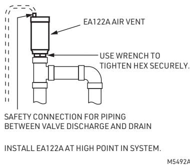
Fig. 3. Install the EA122A at high point in system.
