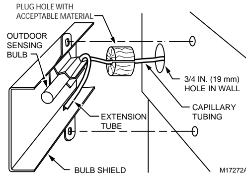
Fig. 16. Mounting bulb in bulb shield.
