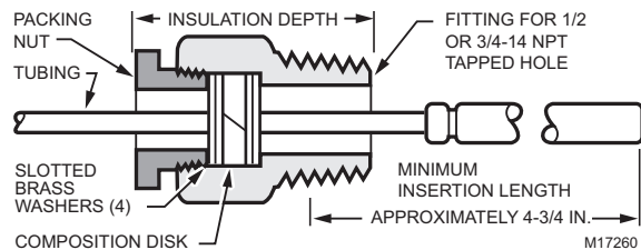
Fig. 1. Capillary compression fitting dimensions and components.
