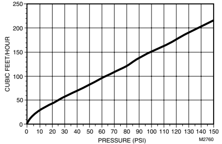
Fig. 2—EA79 flow capacities, with leakage guard cap.
