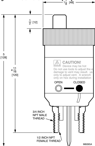
Fig. 1—EA79 dimensions in in. [mm].
