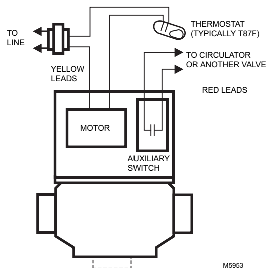
Fig. 14. Typical wiring for V8043E, V8044E.
