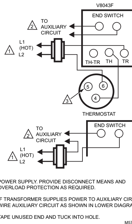
Fig. 35. Wiring a Honeywell V8043F to a White-Rodgers System (alternate option).
