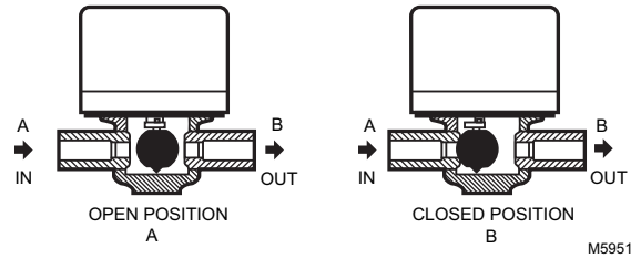
Fig. 36. V8043 operation for normally closed valve.
