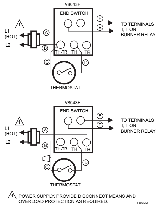
Fig. 31. Wiring a Honeywell V8043F to a Flair System (two options). (Wires are identified with letters to correspond with wires on Fig. 29.)
