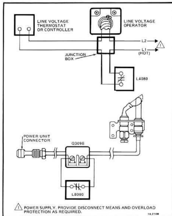
Fig. 4—Typical wiring hookup for line voltage system.
