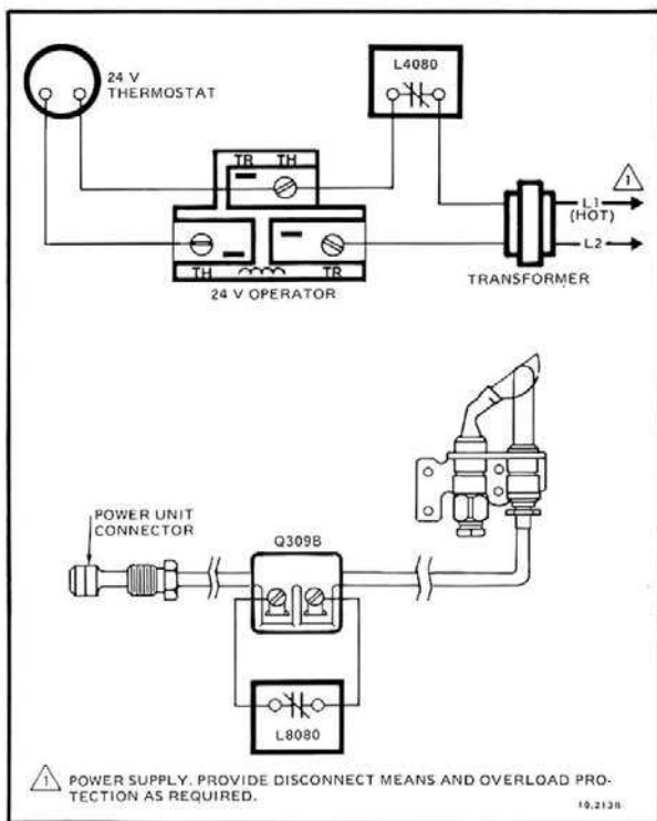
Fig. 3—Typical wiring hookup for 24 V systems.
