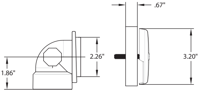
Faceplate
