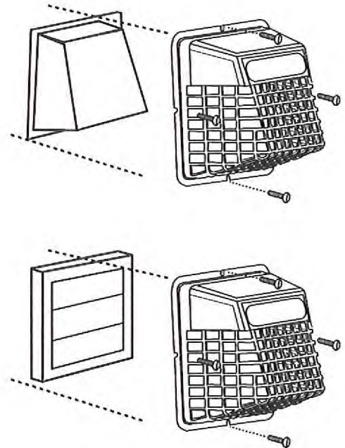
Application View
