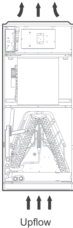
Fig. 7 – Vertical Upflow Installation
