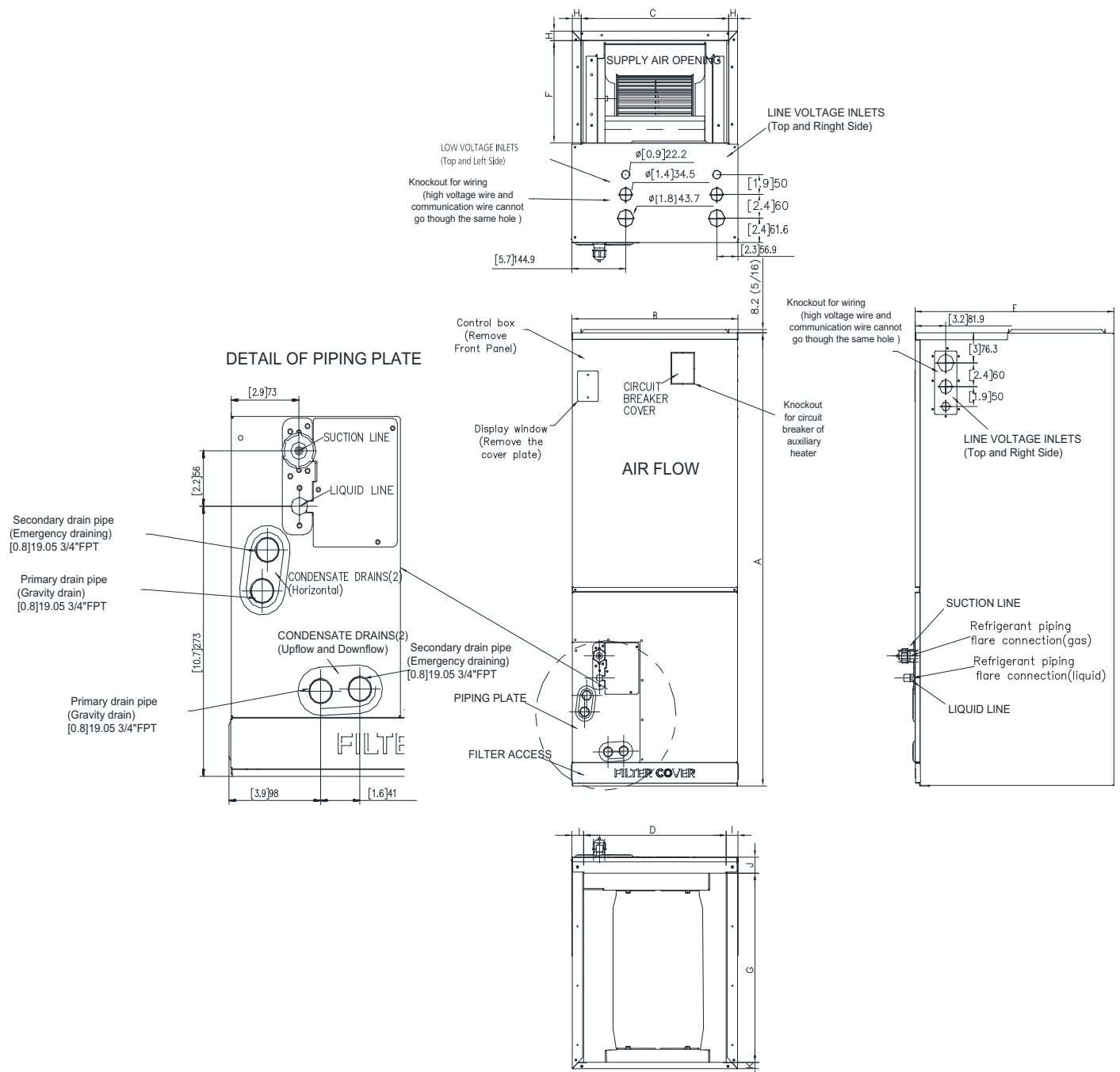
Fig. 11 – Dimensions 18K – 60K, (in.)mm
