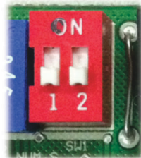
Fig. 24 – Micro-Switch SW1
