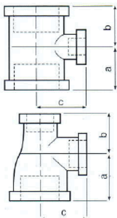
Reducing Tee
