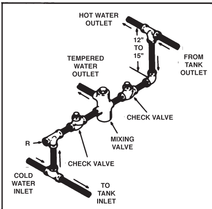
MIXING VALVE APPLICATION FOR TWO TEMPERATURE SYSTEM
