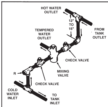
MIXING VALVE APPLICATION FOR TWO TEMPERATURE SYSTEM
