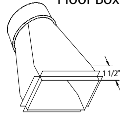
Floor Box
