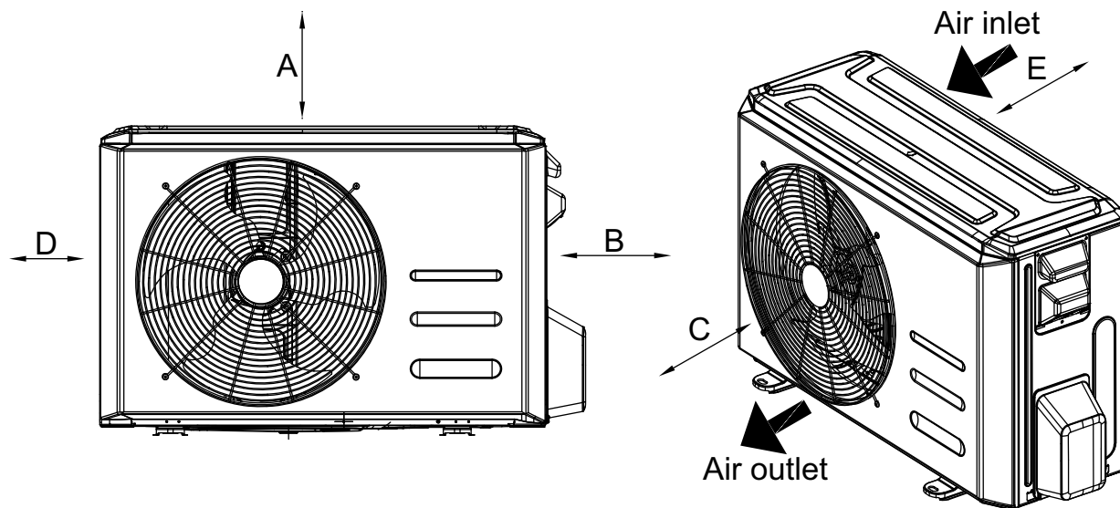
Fig. 6 — Clearances
