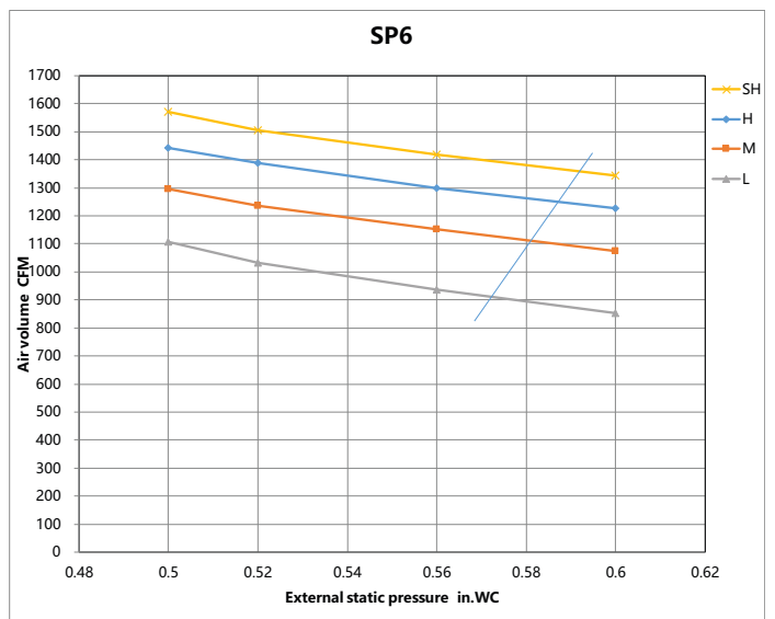
Fig. 30 – High Static Pressure Curves - 36k
