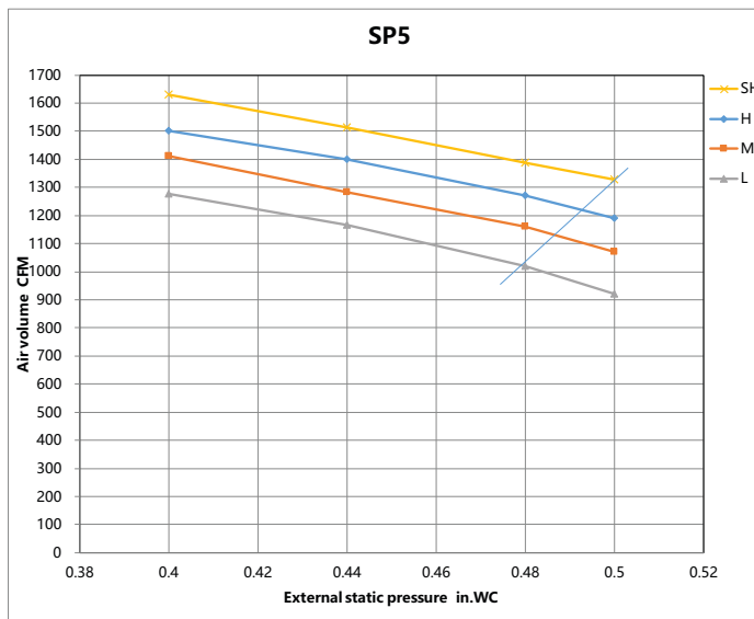
Fig. 30 – High Static Pressure Curves - 36k
