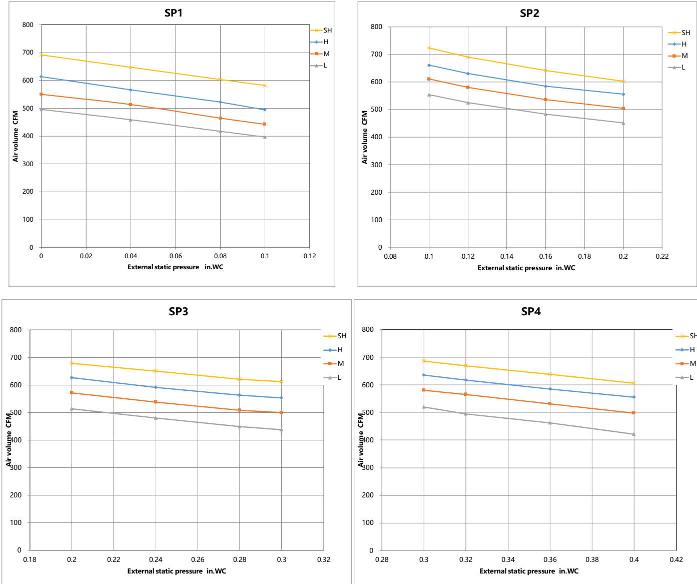
Fig. 19 – Low Static Pressure Curves – 18k
