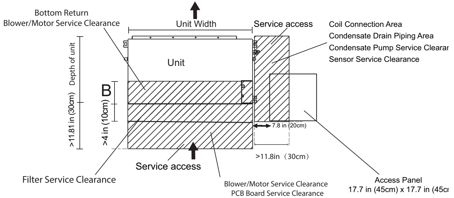
Fig. 9 – Maintenance Clearance
