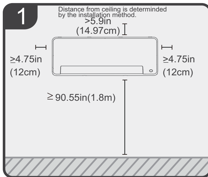
Fig. 3 – Indoor Unit Clearances
