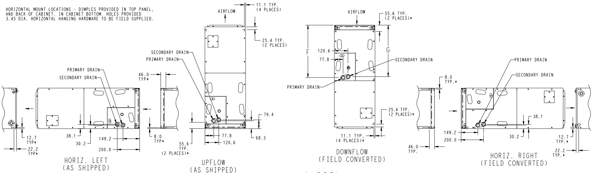
Fig. 4 – FCMA5 Dimensional Drawing, sheet 4
