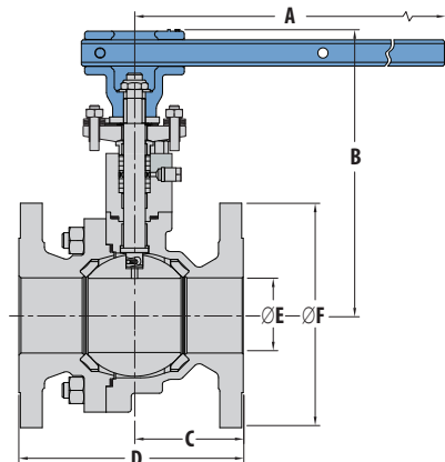
Full port, live-loaded, and double packed
