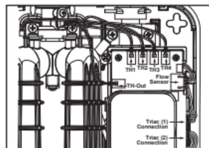
Figure 34 - Sensors control board terminal locations.
