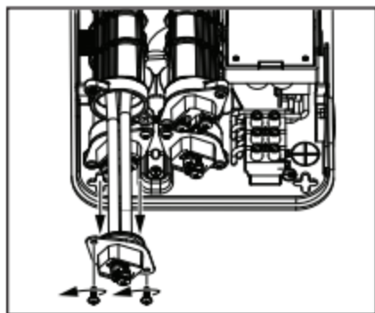
Figure 13 - Removing the element(s).
