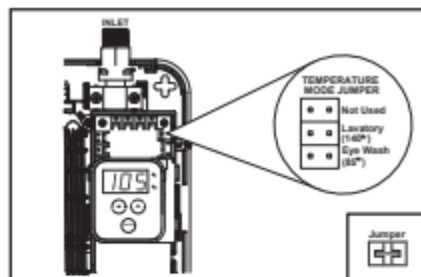
Figure 6 - Temperature mode jumper.
