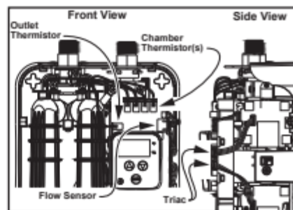
Figure 46 - Control Board Component Connections
