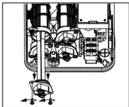
Figure 20 - Removing the element(s).
