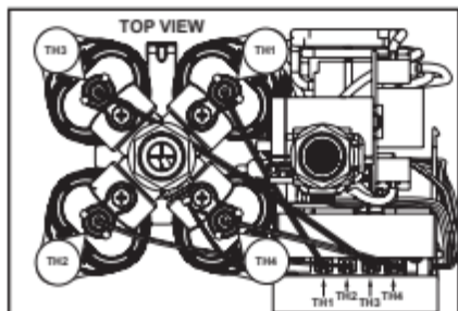
Figure 35 - Thermistor wire configuration.
