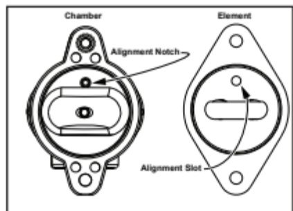
Figure 21 - Chamber Alignment Notch, Element Slot.
