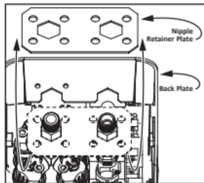
Figure 32 - Nipple retainer plate removal.
