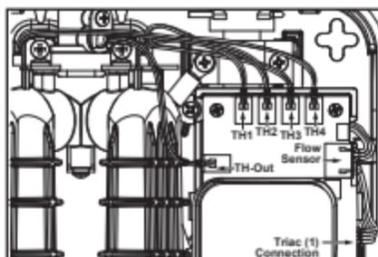
Figure 28 - Sensors control board terminal locations.
