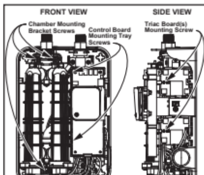
Figure 36 - Mounting screw locations.
