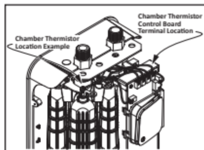
Figure 25 - Chamber thermistor location.
