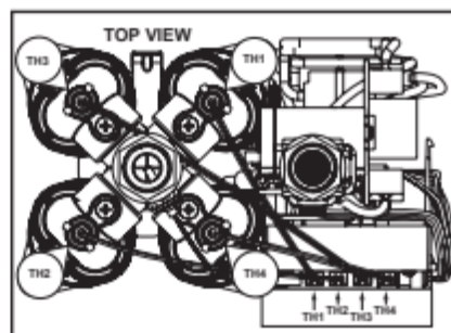
Figure 26 - Proper chamber thermistors installation.
