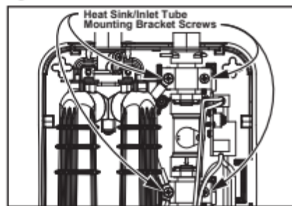
Figure 31 - Heat-sink/inlet tube mounting bracket screws.
