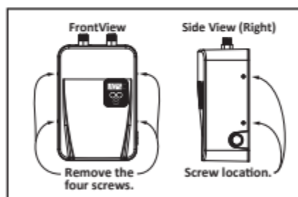
Figure 5 - Removing the front cover.
