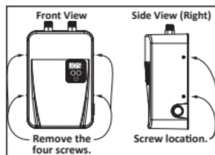
Figure 11 - Accessing Point-of-Use Control Board
