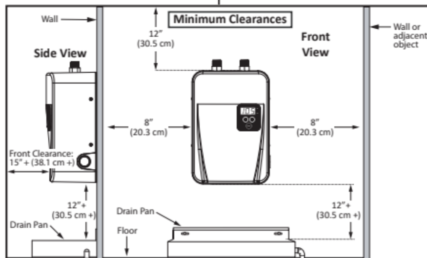
Figure 2 - Clearance Specifications
