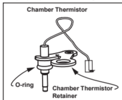
Figure 27 - Chamber thermistor with o-ring.
