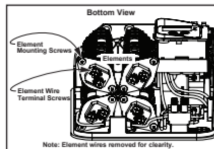
Figure 12 - Bottom view, element(s).
