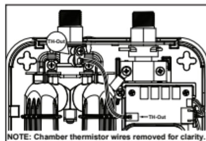
Figure 23 - Proper outlet thermistor installation.
