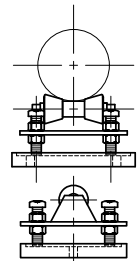
Figure 40 Adjustable Chair and Roll Page 129
