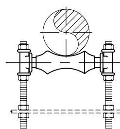
Figure 109 & 109 SS316 Adjustable Roll Support Page 138
