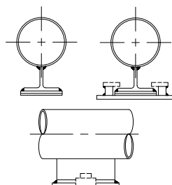
Figure 1010 Pipe Slide Assembly Page 146
