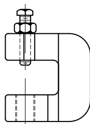
Figure 196 C-Clamp with Locking Nut (Malleable Iron) Page 68
