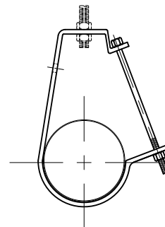
Figure 967J & 967JF & 967J PVC Extension Ring Hanger Page 30
