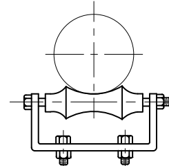
Figure 54 Roller Chair Page 128
