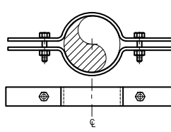
Figure 126LD & 126LD PVC Light Duty Riser Clamp Page 48
