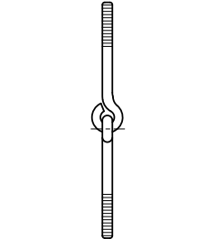
Figure 306 & 341 Linked Eye Rods (Welded & Not Welded) Page 98
