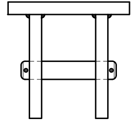
FIGURE 113B FOR ROD SIZES 2" THRU 3 1/2"
