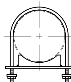
Figure 127 Anchor Chair Page 61
