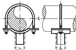
Figure 125 Pipe Saddle with U-Bolt Page 110
