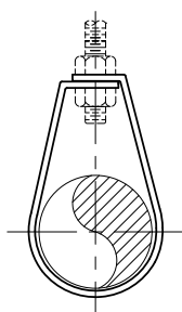
Figure 1A CE Copper Tubing Band Hanger Page 26
