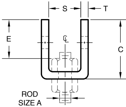
FIGURE 113A FOR ROD SIZES 3/8" THRU 1 3/4"
