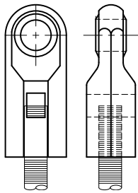
Figure 157 Extension Piece Page 106
