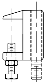
Figure 192W Wide Mouth Top Beam Clamp with Locking Nut Page 70
