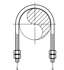
Figure 283 SS & 283 SS316 Stainless Steel U-Bolt Page 56
