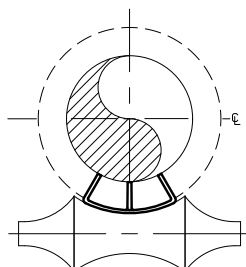
Figure 351 thru 357Z Pipe Covering Protection Saddle Page 116
