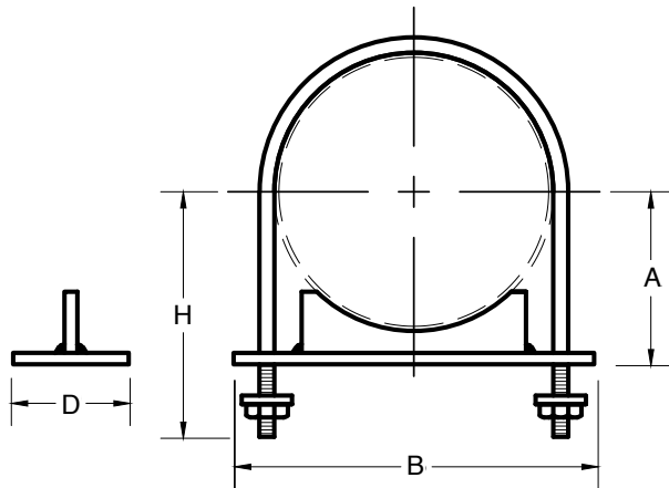
FIGURE 127 - ANCHOR CHAIR
