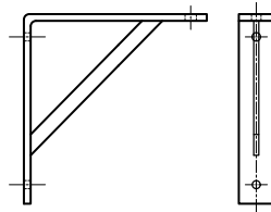
Figure 69 Light Welded Steel Bracket Page 81
