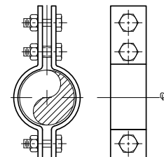
Figure 304 Three Bolt Pipe Clamp Page 36
