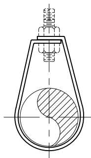
Figure 1A, 1A PVC Band Hanger Page 25
