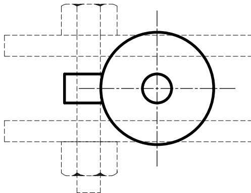
FIGURE 258 - SOCKET CLAMP WASHER
