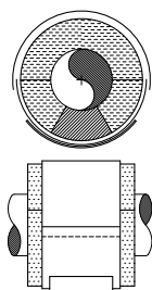
Figure 465CVB-MSRH High Point Load Calcium Silicate Insulation Shield Page 152
