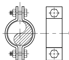
Figure 298 Heavy Duty Two Bolt Pipe Clamp Page 35
