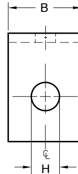
FIGURE 113B FOR ROD SIZES 3/8" THRU 1 3/4"
