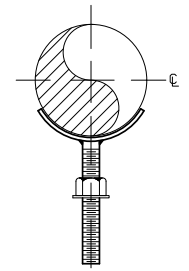
Figure 137 Adjustable Pipe Support Page 112
