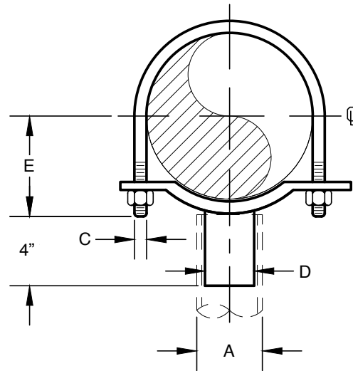
FIGURE 125DI - PIPE SADDLE WITH YOKE FOR DUCTILE IRON AND CAST IRON PIPE
