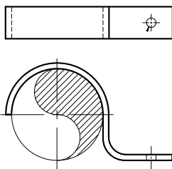
Figure 237 One Hole Pipe Clamp Page 57
