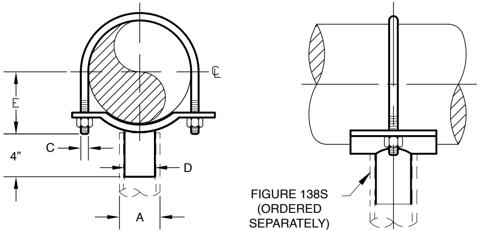
FIGURE 125 - PIPE SADDLE WITH YOKE
