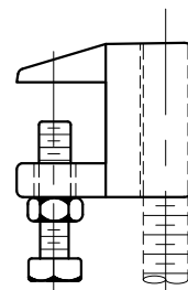
Figure 192 & 192 SS316 Top Beam Clamp with Locking Nut Page 69
