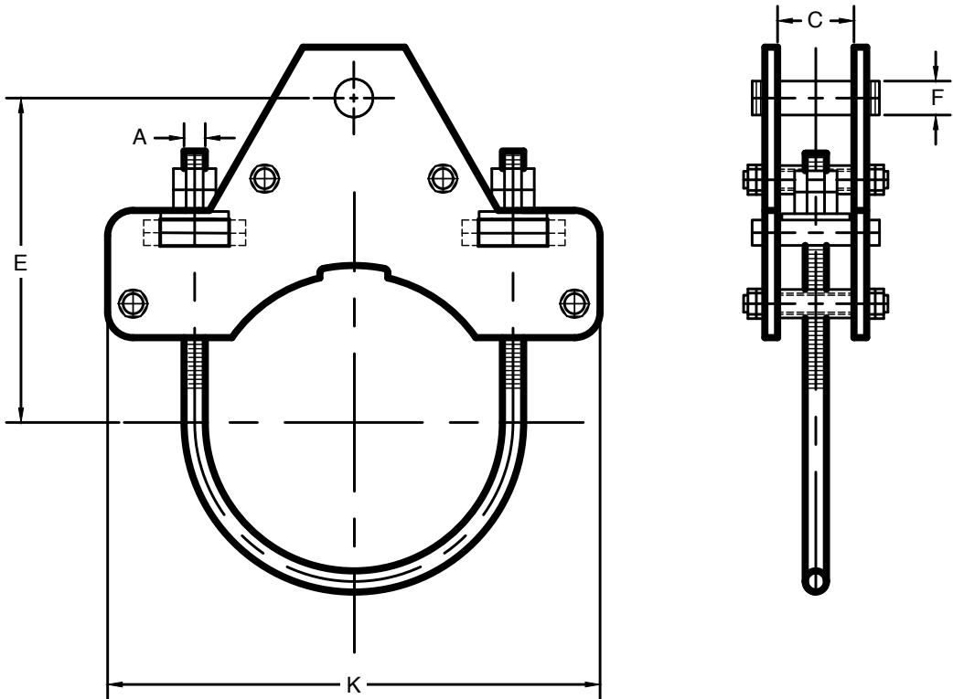
FIGURE 134 - STANDARD ALLOY YOKE CLAMP
