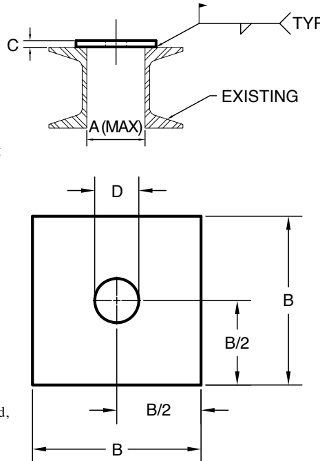
FIGURE 260 - WASHER PLATE
