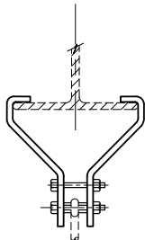
Figure 314 Extended Beam Clamp Page 74
