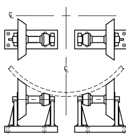
Figure 6718 Large Diameter Fabricated Pipe Roll Page 140
