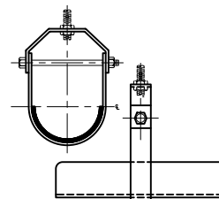
Figure 100SH Clevis Hanger with Shield Page 19
