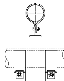
Figure 1015 Heat Trace Pipe Shoe Page 147
