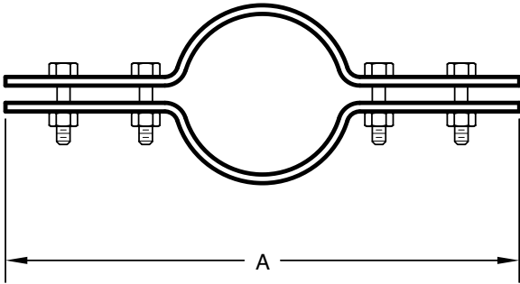
FIGURE 158DB - DOUBLE BOLT DUCTILE IRON PIPE CLAMP
