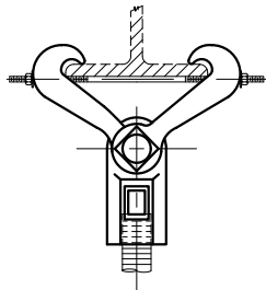
Figure 82 Adjustable Beam Clamp (Body Only) Page 73
