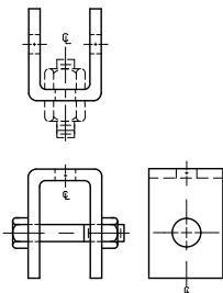
Figure 113A & 113B Welded Beam Attachment Page 86
