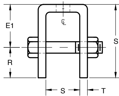
FIGURE 113B FOR ROD SIZES 3/8" THRU 1 3/4"
