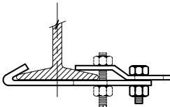
Figure 217 Adjustable Side Beam Clamp Page 77
