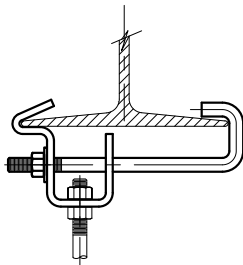
Figure 14 & 14A Adjustable Beam Clamp Page 72
