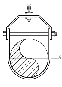
Figure 100 & 100F & 100PVC Plain, Felt Lined, PVC Coated Clevis Hangers Page 13
