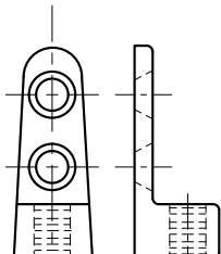
Figure 153 & D153S Side Beam Connector Page 94
