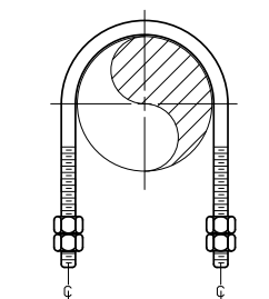
Figure 283HS High Strength U-Bolt Page 54
