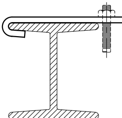
Figure 6 Top Beam Clamp Page 78
