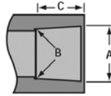
SCHEDULE 80 SOCKET DIMENSIONS ASTM D 2467
