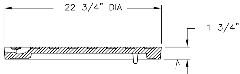
COVER SECTION
