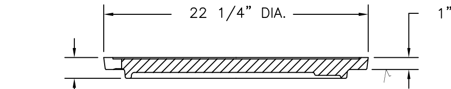
COVER SECTION
