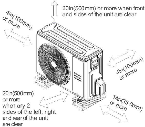
Fig. 5 – Clearances
