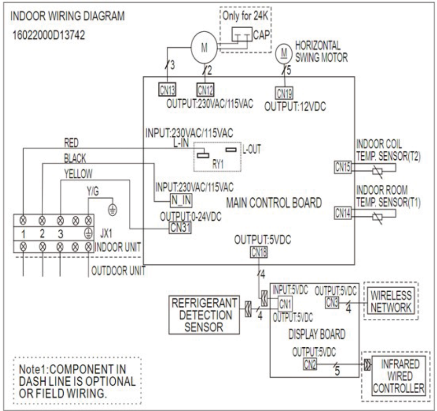
Fig. 7 – Sizes 09 – 24K, with Refrigerant Detection Sensor
