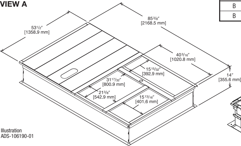
VIEW A
