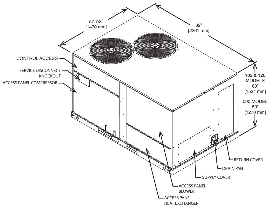
Illustration ST-A1273-26_B-00
