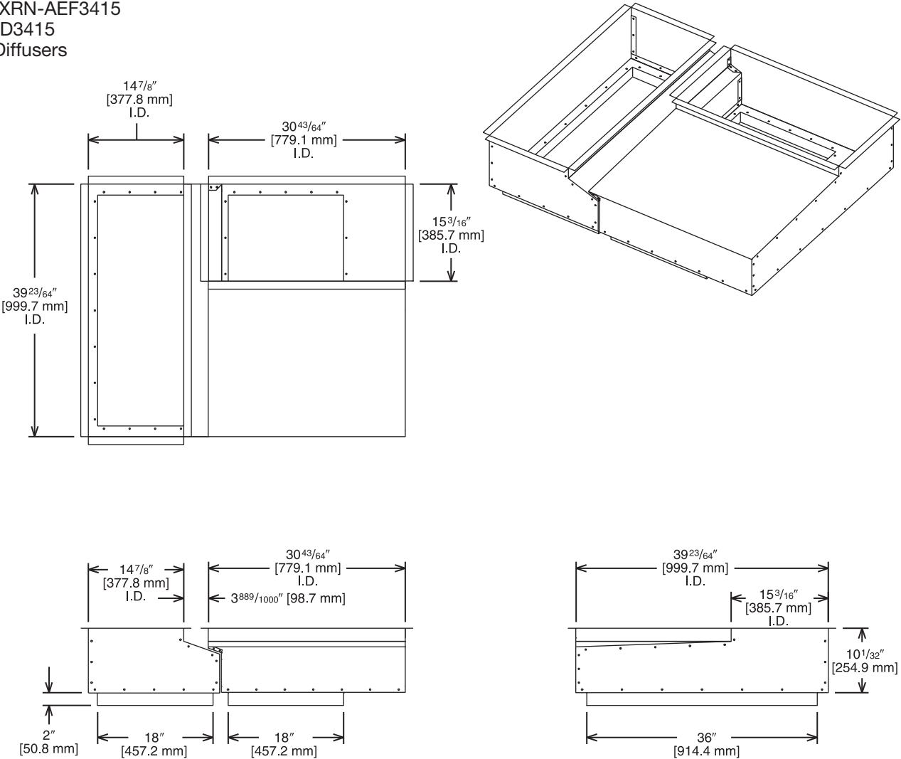
Illustration ADS-106193-03
