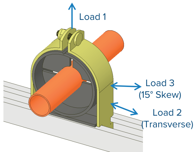
Strut Mounted Coupling for 1/2" Wall Insulation
