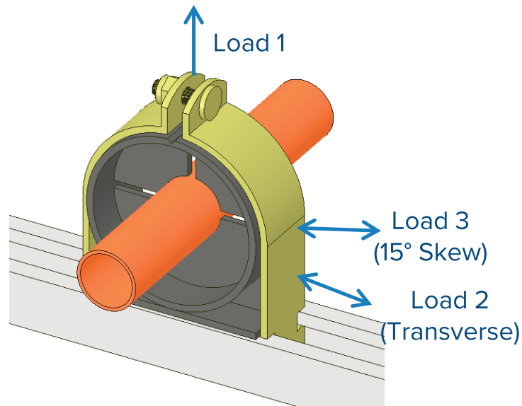
Strut Mounted Coupling for 1" Wall Insulation
