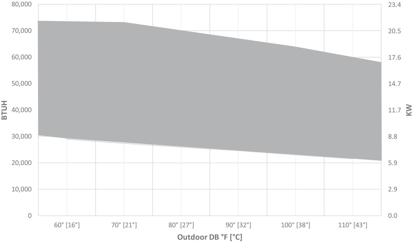
(-)P19AY60 Cooling Capacity Ranges
