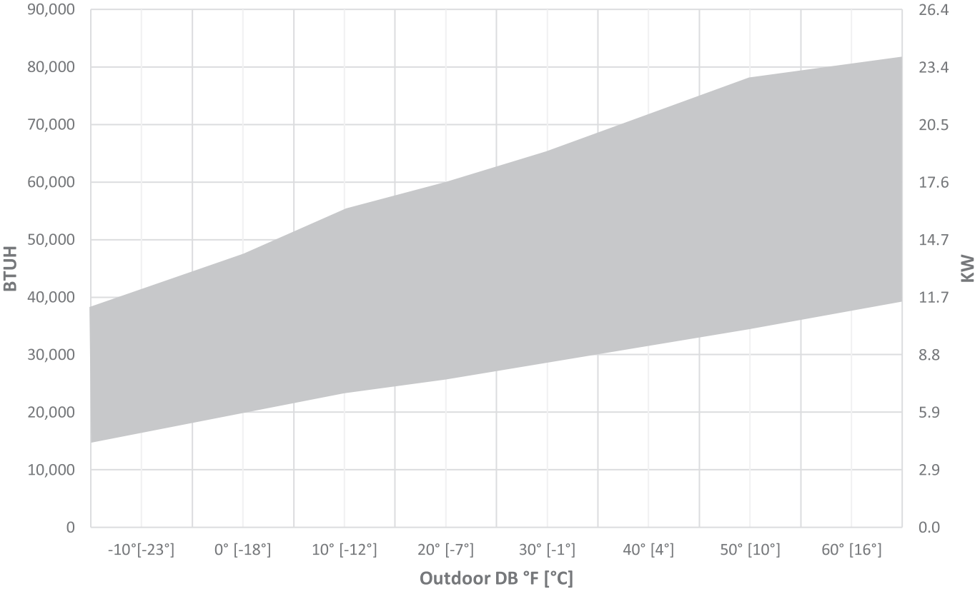
(-)P19AY60 Heating Capacity Ranges
